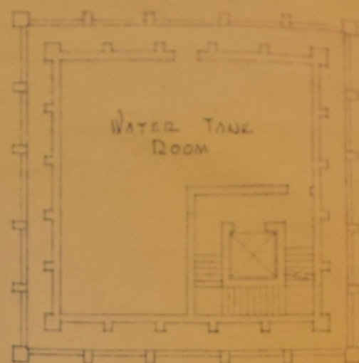
TOWER THIRD FLOOR PLAN
