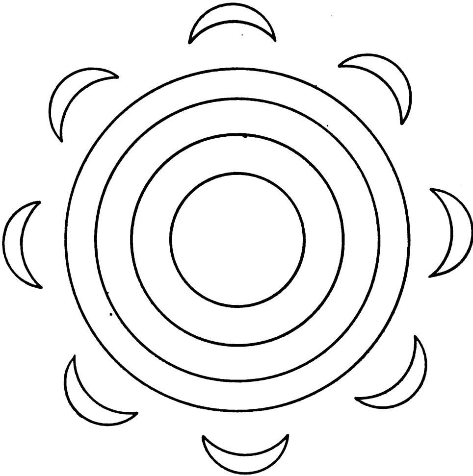
Saturn
