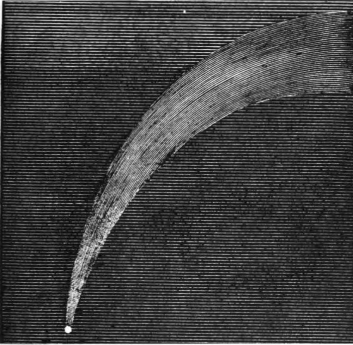
DONATI'S COMET, 1858
