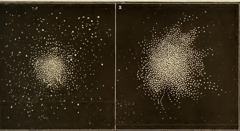
Stellar Clusters.
