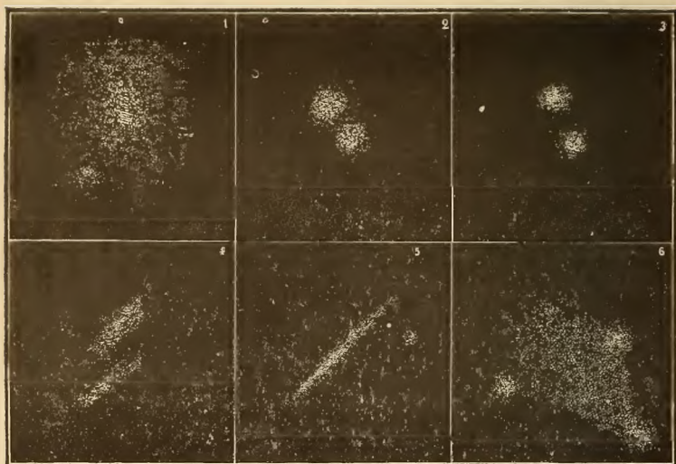
Double and Multiple Nebulae.
