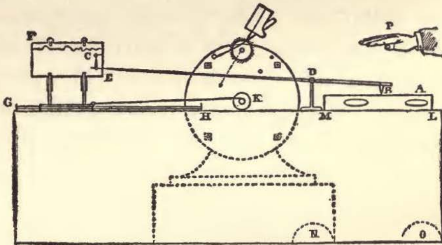
FIG. 17. SECTION OF APPARATUS IN FIG. 16.
