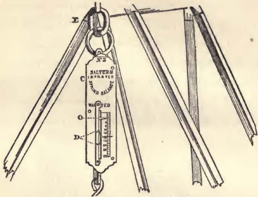
FIG. 10. CROOKES' APPARATUS.
