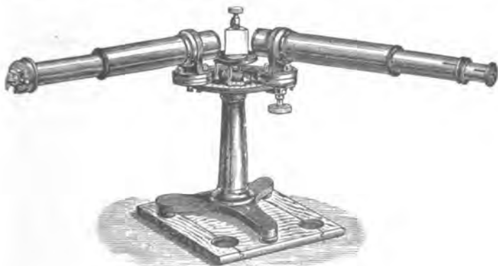
DIAG. 9. — SPECTROSCOPE.
