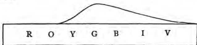
DIAG. 13. — PHOTOGRAPHIC RANGE FOR SILVER SALTS.
