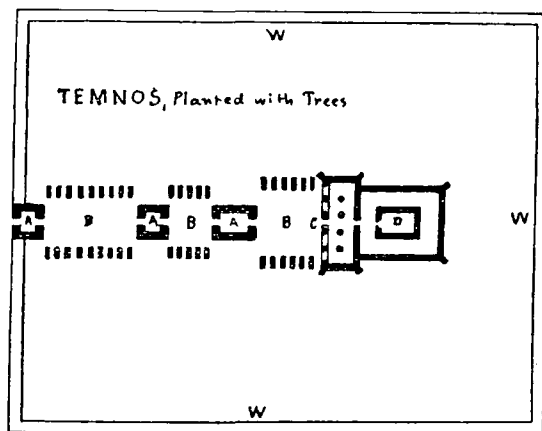
GENERAL PLAN OF AN EGYPTIAN TEMPLE.
