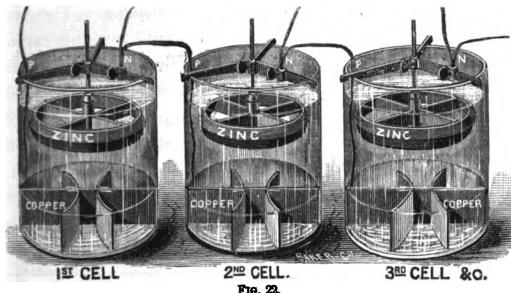
FIG. 22. GRAVITY CELLS. Capacity, \frac{1}{2} Gallon.
