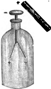
FIG. 7. ELECTROSCOPE. Ht. 12 in. Diam. 4\frac{1}{4} in. in a nickel-plated brass disc.
