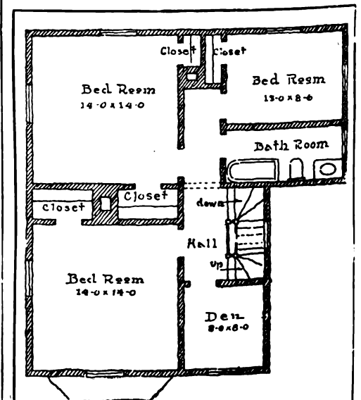
Figure 2.—The second floor plan of a house
