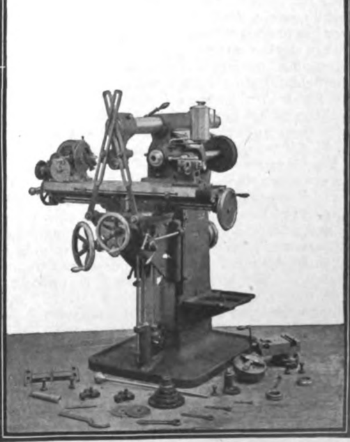
The milling machine quickly and accurately shapes the various sections of intricate modern mechanisms like the Mergenthaler linotype
