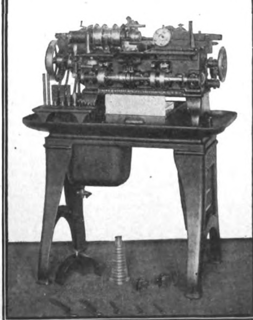
The automatic screw machine cuts small turned parts from metal rods, for watches, clocks, typewriters, etc., twenty every minute
