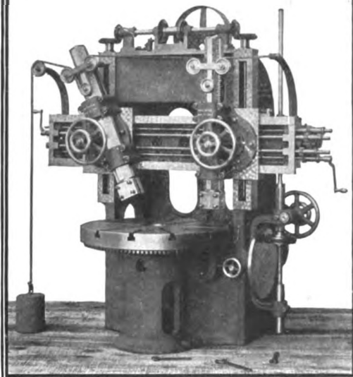
The boring and turning mill turns large fly wheels and driving wheels, taking many hours to make one cut through the hard metal
