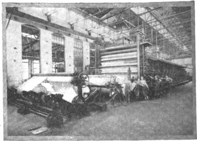
WINDING THE ROLLS FOR THE BIG DAILY PAPERS
