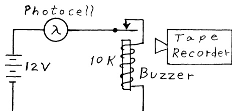
Fig.1 - Signal Recording Circuit
