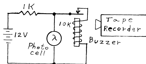
Fig.2 - Revised Circuit
