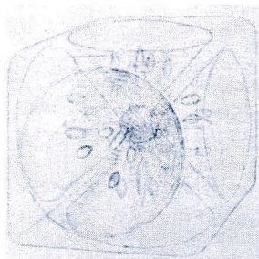
CUBE Boron
