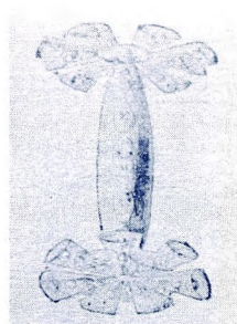
DUMB-BELL Sodium
