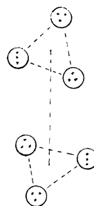
Fig. 4. HYDROGEN ATOM
