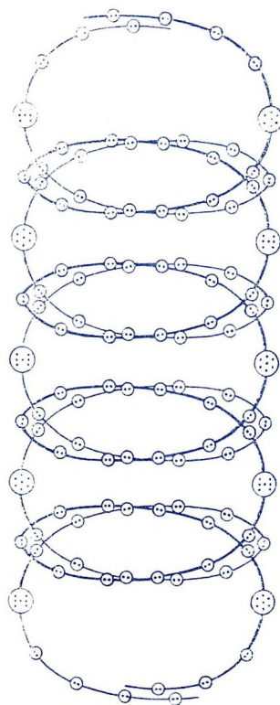
Figure 3. Oxygen Atom
