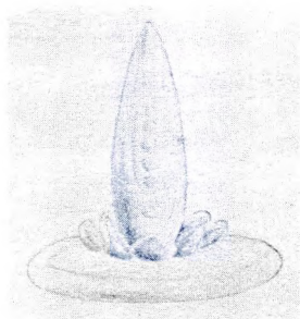
SPIKE Lithium
