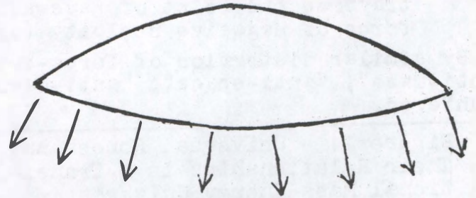
Figure 13A - Theoretic Course of Bottom Sphere-segment's Unaffected Radiant Magnetic Fields and Light. (Excerpt)
