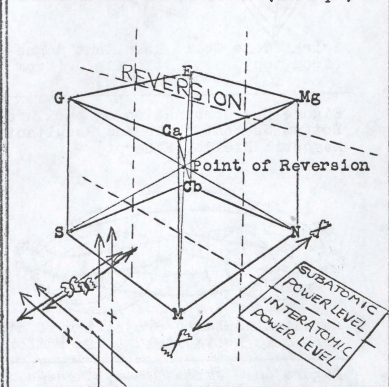
Figure 12 - Universal Forces and Their Relationships in a Reversional-Transitional Cosmos (Excerpt)
