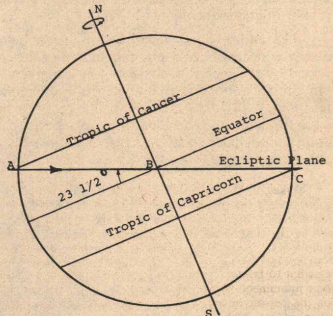
Fig. 2. Arrow shows flight path for satellite launched toward the east at a point A on the Tropic of Cancer when the launch point touches the ecliptic plane.
