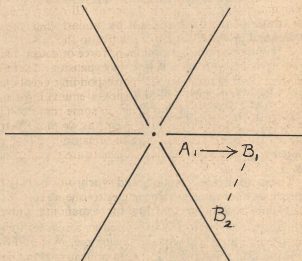
Fig. 1. Dot at center represents the primordial point from which the "big bang" originated. Lines represent the uniform expansion of the universe away from that point in space-time. Since the differentiation of matter and energy is duplicated along each line, similar events on adjacent lines are synchronistic although not causally related ( B_1 \dots B_2 ). Causality is represented by successive events along the same line of expansion ( A_1 \longrightarrow B_1 ).
