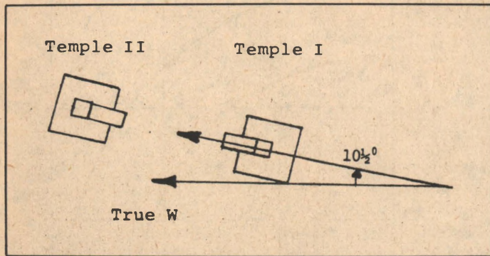
Fig. 5. Orientation of the main temples at the Great Plaza, Tikal.
