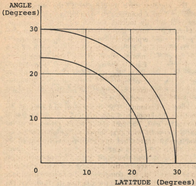
Fig. 3. Angle at which satellite path crosses parallel of latitude for easterly launch, assuming non-rotating Earth.
