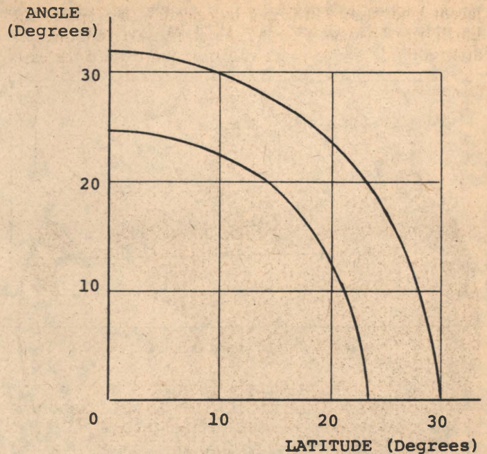
Fig. 4. Angle at which satellite path crosses parallel of latitude for easterly launch, allowing for Earth's rotation.
