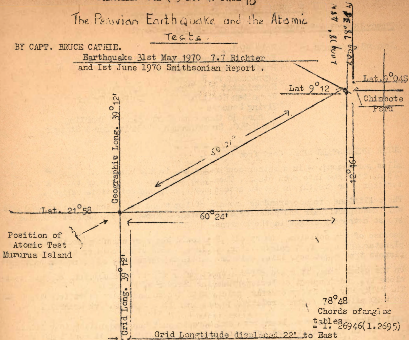
DIAGRAM SHOWS CORRELATION BETWEEN ATOMIC TESTS AND EARTHQUAKES.
