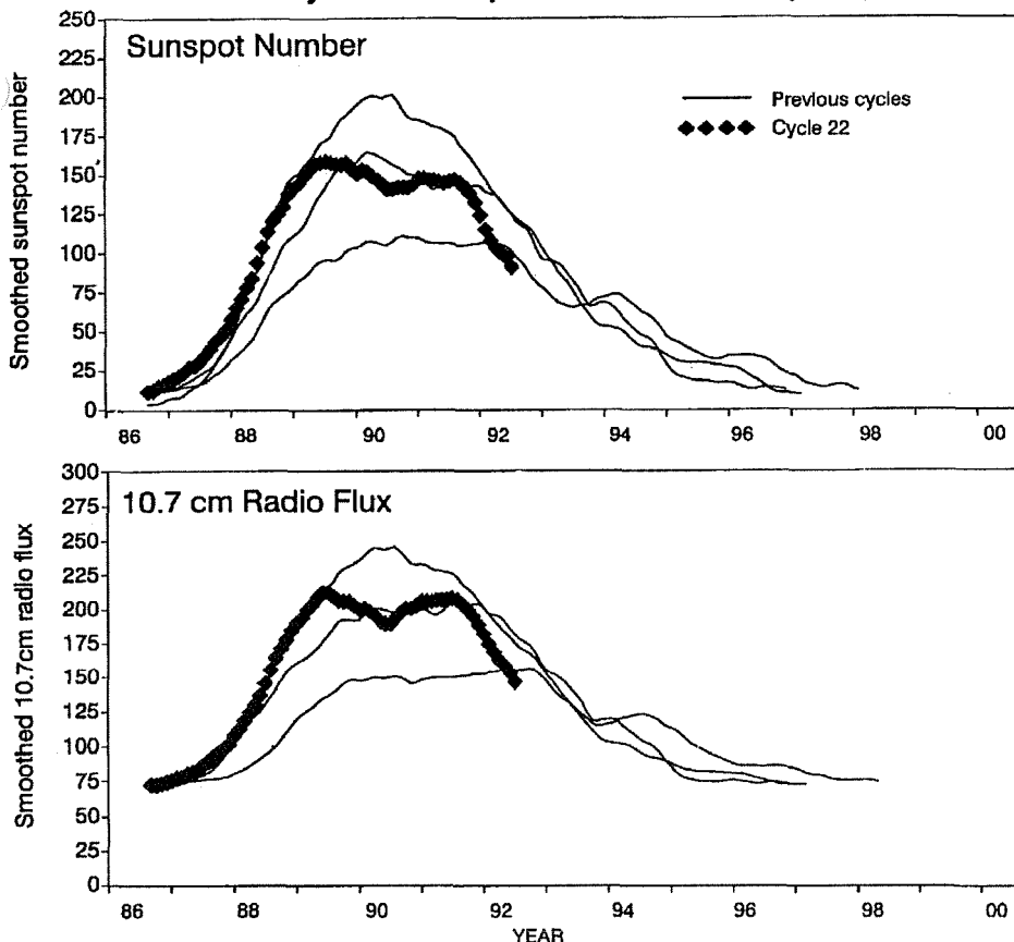
Solar Cycle 22 Compared to the last 3 Cycles
