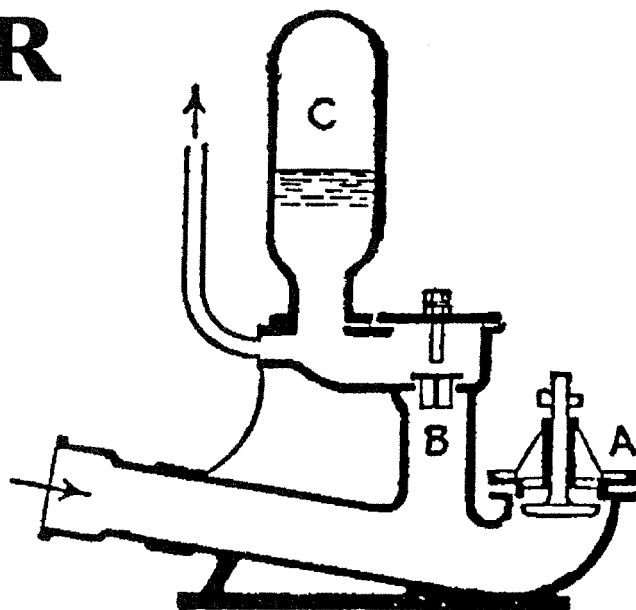
Figure 6 HYDRAULIC RAM PUMP
