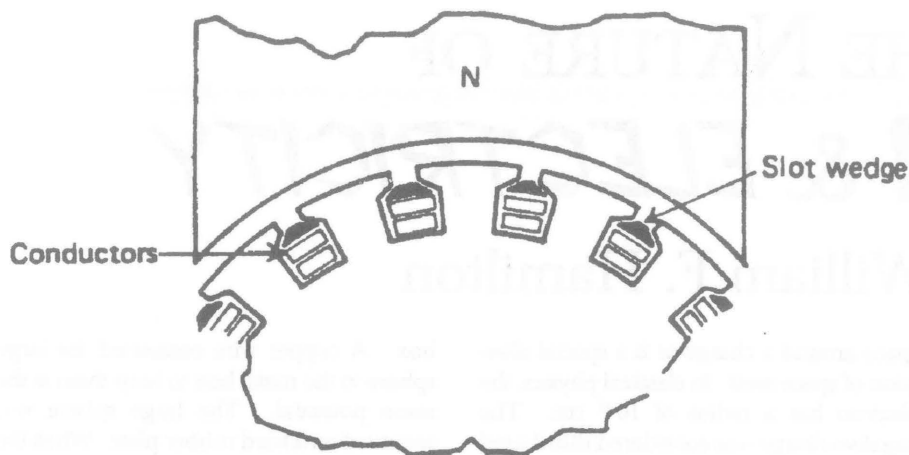
figure 5 Rotor conductor arrangement in a modern machine.
