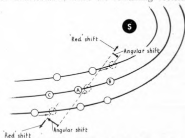
Fig. 4. Orbital cosmos theory of the expanding universe.
