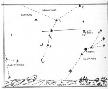
Fig. 1. The sky above the southern horizon at 22.00 hrs. G.M.T. on August 5, 1957.
