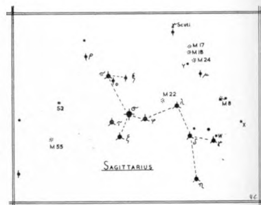
Fig. 3. The Constellation Sagittarius (The Archer).
